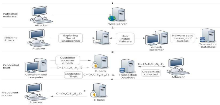
Figure 3: Credential Theft
