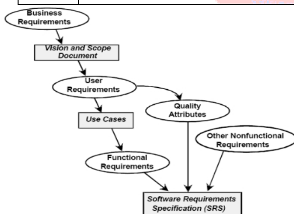
Fig :2 Software Requirements Specification
